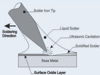
Figure 1. Illustration of Ultrasonic Cavitation Removing Surface Oxides in a Solder Joint
